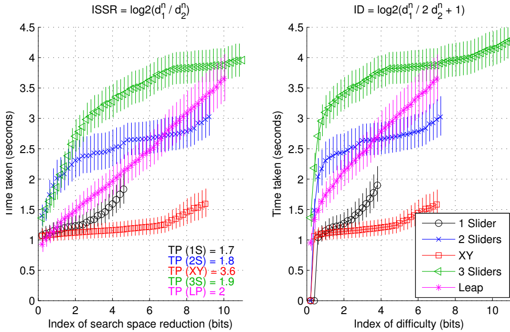
Figure 7.11: ISSR plot for the visible target condition (left) the kinks in the plots for the sliders are caused by having to swap controls. If we imagine the curves extrapolated onwards to higher accuracies, it seems that the 3 sliders will overtake the Leap. The right hand plot uses MacKenzie’s ID, introducing sharp drops at low IDs.
