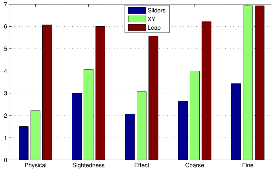
Figure 7.15: User ratings for difficulty of various aspects of the task: Physical effort, ability to know which direction to travel in (i.e. sightedness), ascertaining the effect of movements on timbre, locating a coarse match, and locating a fine match.
