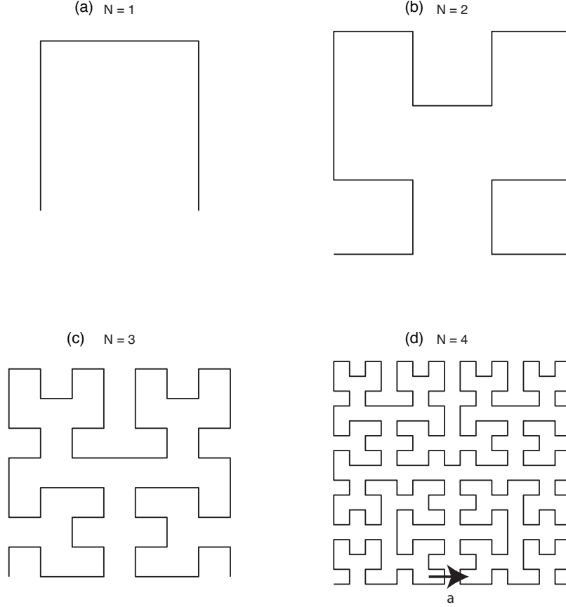
Figure 6.3: Four iterations of Hilbert curve construction in two dimensions. Arrow a demonstrates a locality violation: a small movement in the 2D plane can result in a large 1D distance along the curve.
