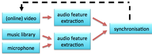
Fig. 3. MuViSync Mobile extracts audio from either the device’s microphone or the device’s music library. Simultaneously, the application streams video content from YouTube, plays music, extracts features and synchronises the video playback in real-time, ensuring the video is synchronised. The algorithm maintains the synchronisation by altering the video as people are more perceptive to jumps in the audio.
